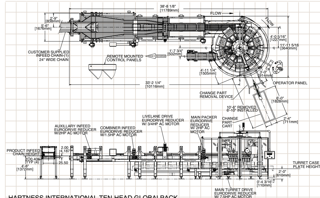
HARTNESS INTERNATIONAL TEN-HEAD GLOBALPACK L.H. MACHINE DRIVE SIDE SHOWN
