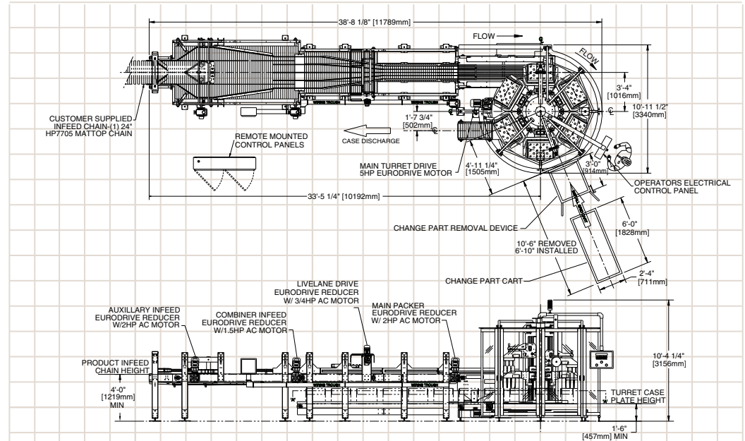
HARTNESS INTERNATIONAL SIX-HEAD GLOBALPACK L.H. MACHINE DRIVE SIDE SHOWN
